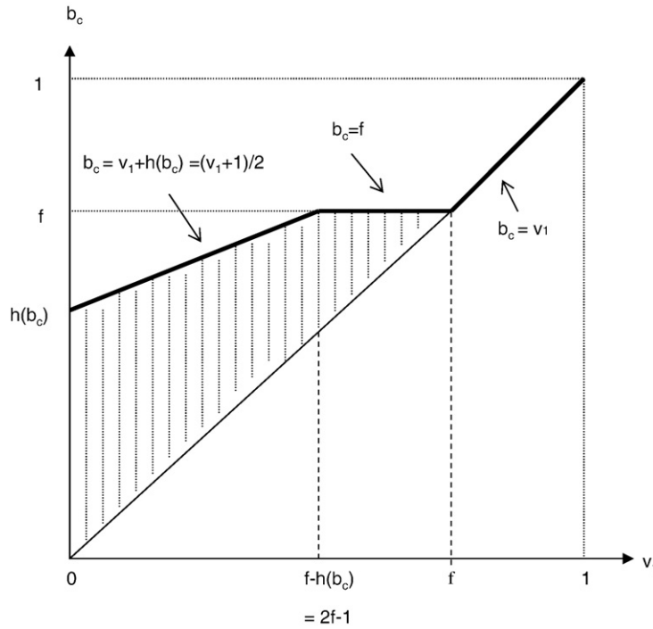
Fig. 1. The bank–bidder coalition's optimal bid, b_c(v_1) , and the expected amount of overbidding (shaded area), assuming a piecemeal liquidation value l of zero. The figure is drawn assuming bidder valuations are distributed uniform, v_1 \sim U[0,1] . The coalition-bidder's private valuation is v_1 , f is the face value of the bank's debt, and h(b_c) is the inverse hazard rate at b_c . When v_1 \leq 2f - 1 , the coalition fully overbids: b_c = (v_1 + 1)/2 . When f > v_1 > 2f - 1 , the coalition partially overbids: b_c = f . When v_1 \geq f , the coalition does not overbid: b_c = v_1 .
