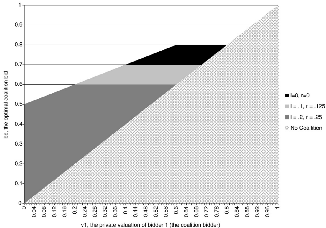
Fig. 3. The expected amount of coalition overbidding for different values of the piecemeal liquidation value l . The figure illustrates how changes in l affect the expected amount of overbidding E(b_c - v_1) , where b_c is the coalition's optimal bid and v_1 is the coalition-bidder's private valuation (distributed uniform). The face value of the bank's debt claim is set to f=0.8 . E(b_c - v_1) equals the shaded area above the diagonal line ( v_1 , bidder 1's optimal bid with no overbidding) and below f-l . As l increases, the bank's liquidation recovery rate r=\min[l/f, 1] increases and E(b_c - v_1) decreases. The figure is drawn for three alternative values of l : l=0.0 , l=0.1 , and l=0.2 . The corresponding expected amounts of overbidding are the shaded areas below f-l=0.8 , f-l=0.7 , and f-l=0.6 , respectively. Thus, the downward shifts in f-l reduce the region for overbidding.
