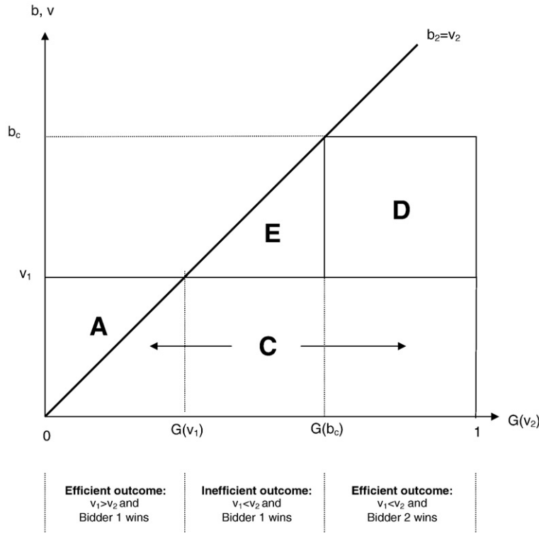
Fig. 2. Expected profits with and without coalition bidding. The figure is drawn assuming bidder valuations are distributed uniform, v_i \sim U[0, 1] . G(v_2) is the cumulative distribution over v_2 . Bidder 2's optimal bid is b_2 = v_2 (the diagonal line) and the coalition's optimal bid is b_c . Area A is the expected profits to Bidder 1 and C is the bank's expected revenue under non-cooperative bidding. With coalition bidding, area E is bidder 1's expected cost of overbidding (the minimum transfer), and area E + D is the bank's expected net revenue from overbidding. Thus, area D is the coalition's expected net surplus from overbidding (which equals the expected wealth transfer from bidder 2).
